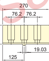
Soft jaw SJ-40~79
