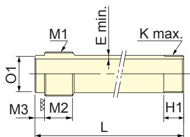
Detail of Draw Tube L = A + G2_{max.} + H - G1_{max.} + M2 + M3
