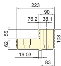
Hardened jaw HJ-40~79
