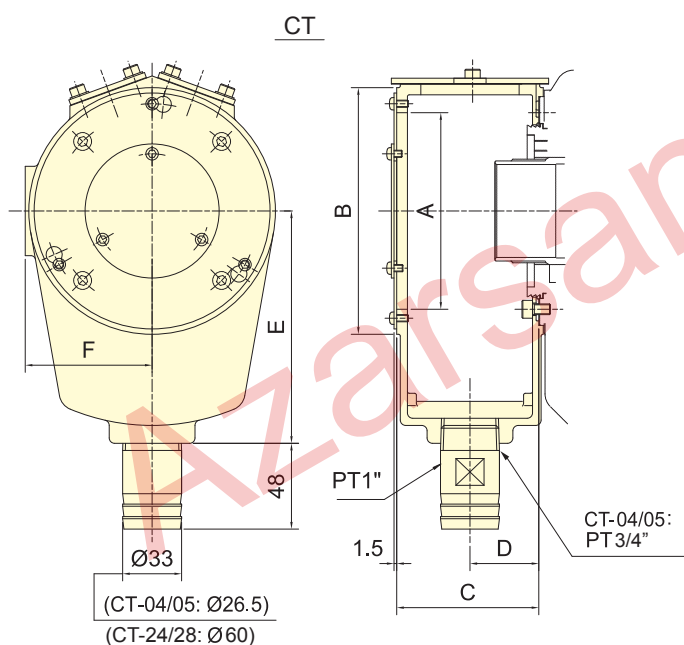
Coolant Collector
