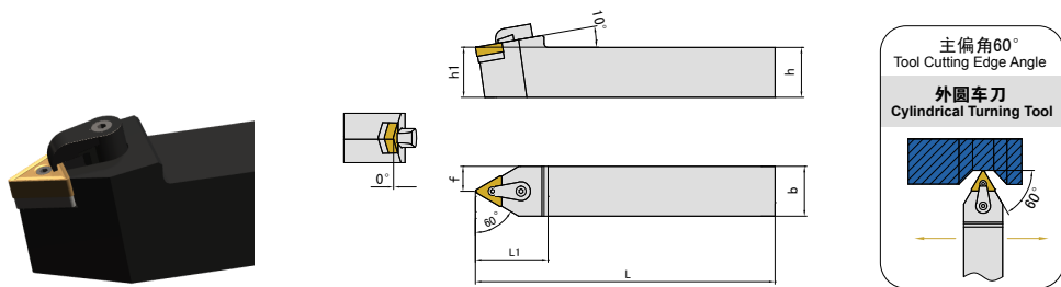
External Turning Tool holder(Negative)
