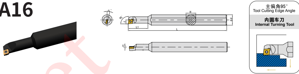
Internal Turning Toolholder
