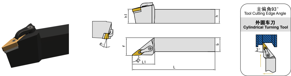
External Turning Tool holder(Negative)
