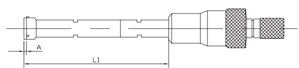
Dimension: 6-12mm / .275-.5"
